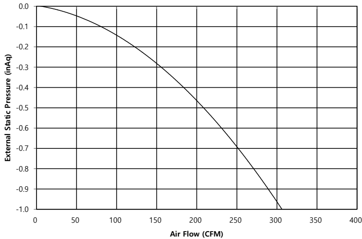
TA Frame Outside Air PTVK410 Ventilation Kit with PTVK420 Flange
