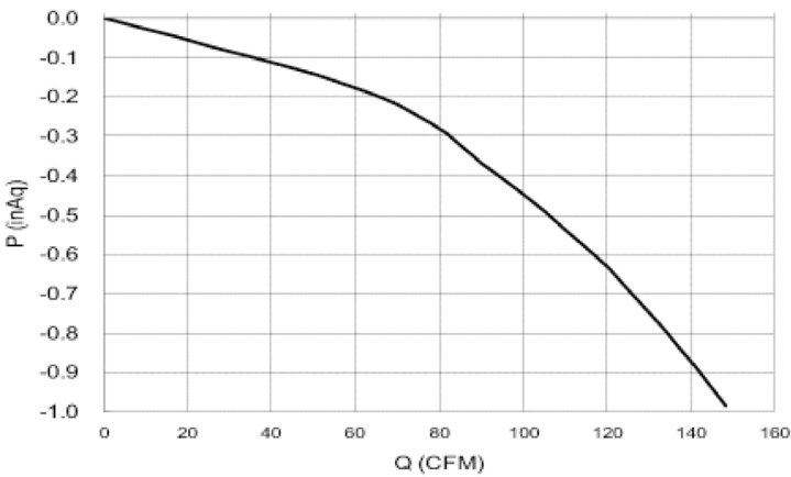
TP, TN, TM Frame Outside Air PTVK410 Ventilation Kit with PTVK420 Flange (Airflow Capacity Versus Static Pressure)
