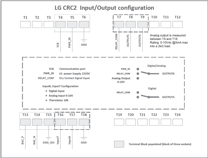
Figure 46: Input/Output Configuration
