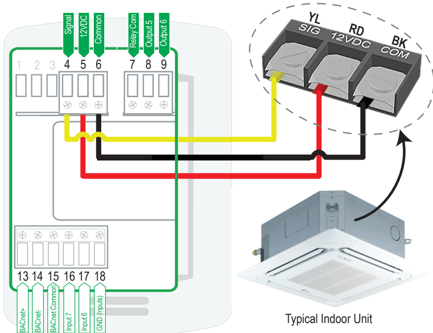
Figure 5: Controller Wiring
