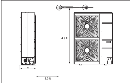
Figure 15: R32 Standard Singe-Zone Systems - A-Coil Outdoor Unit Sound Pressure Level Measurement Location (For Illustrative Purposes Only; Appearance Depends on Model).
