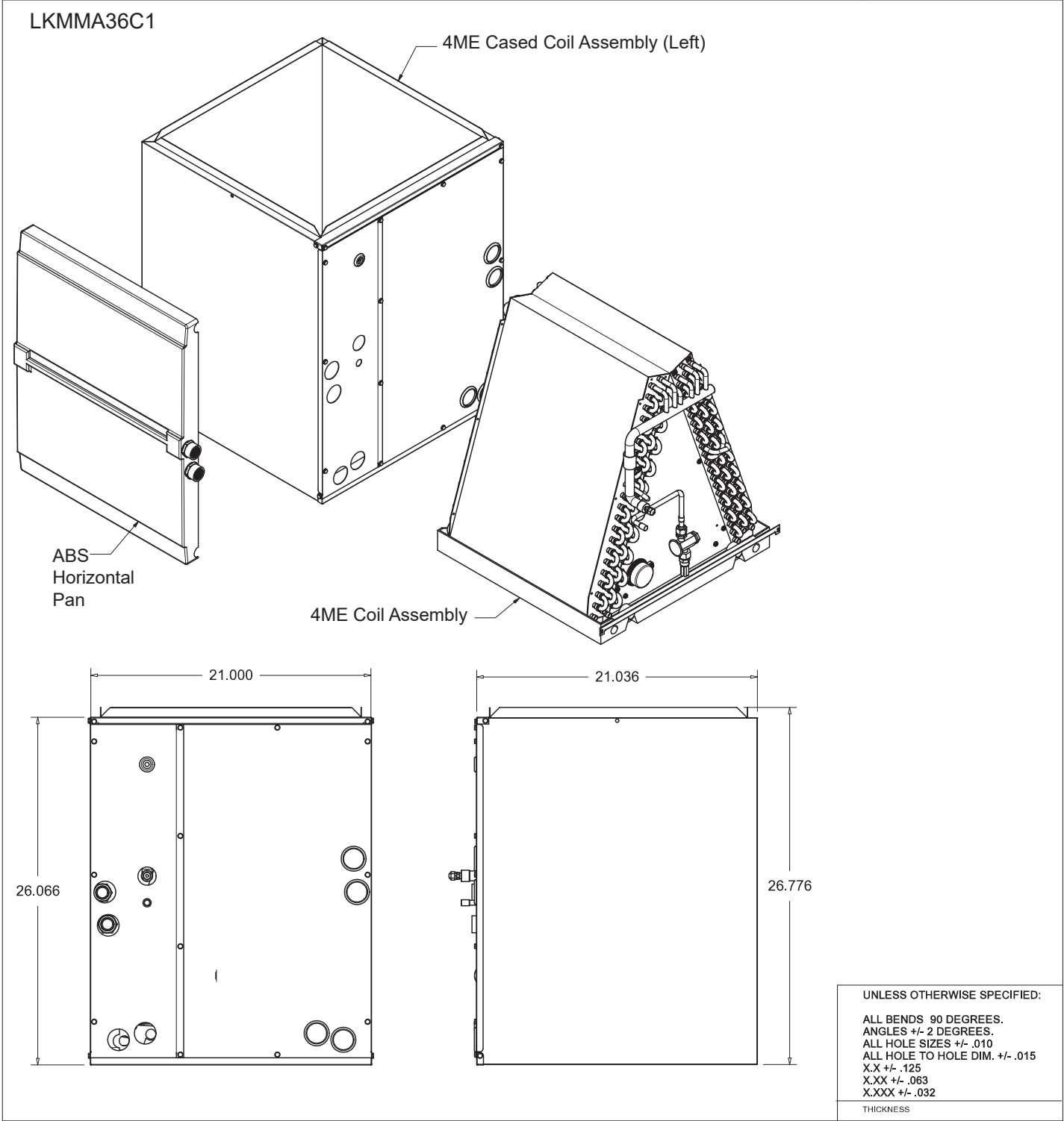
Figure 12: LKMMA36C1 A-Coil Unit Dimensions.
