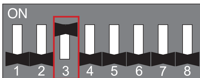
Figure 57: SW-01 DIP Switch Heat Pump Communication Kit Setting for A-Coil / Third-Party Furnace.
