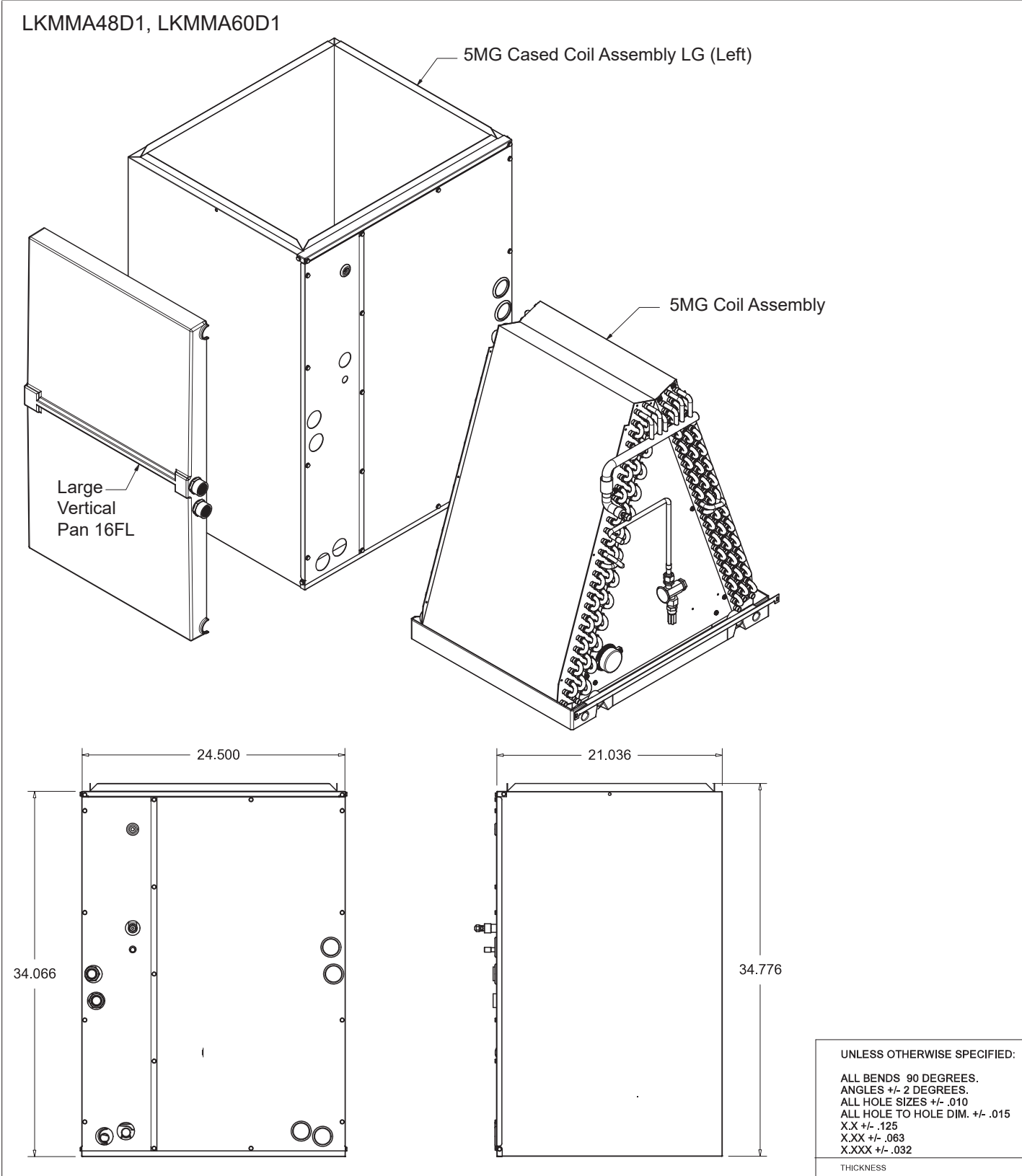
Figure 14: LKMMMA48D1, LKMMMA60D1 A-Coil Unit Dimensions.
