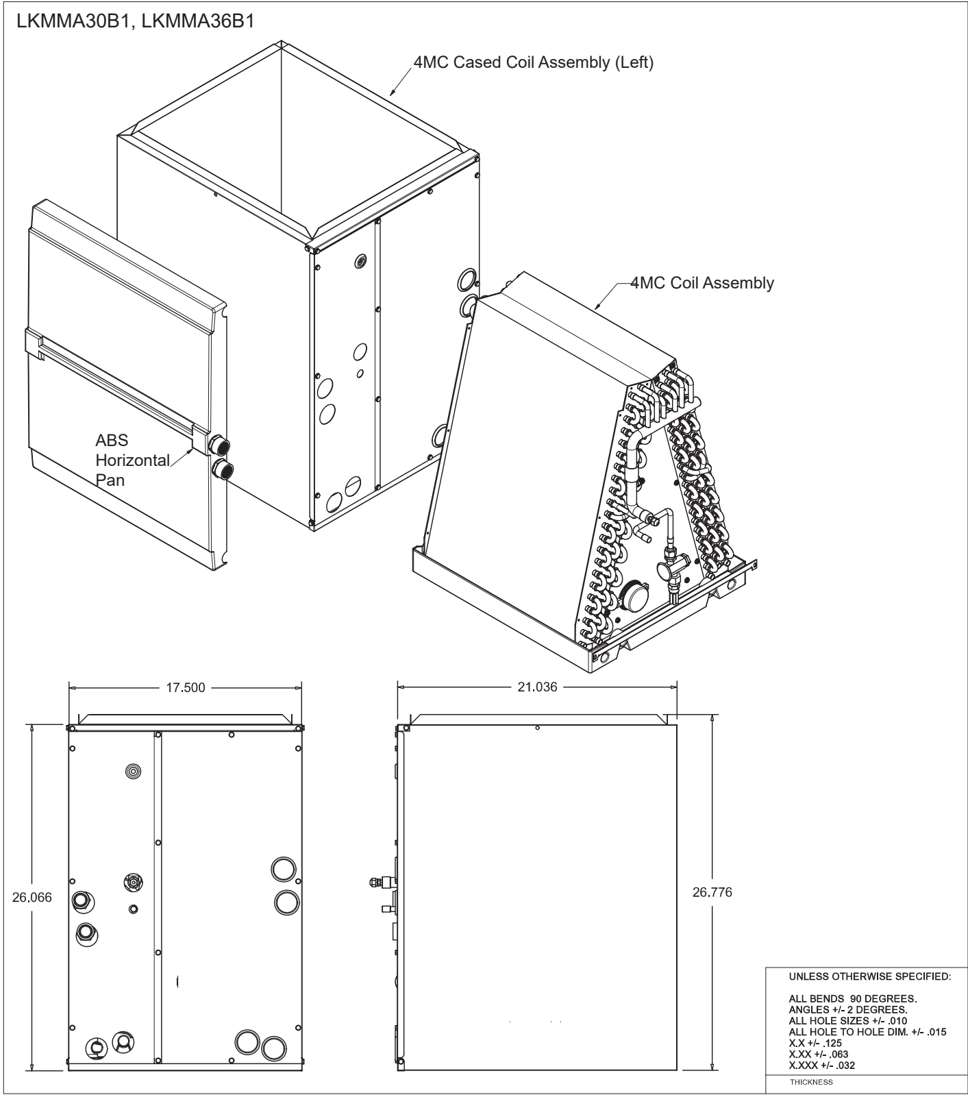
Figure 11: LKMMA30B1, LKMMA36B1 A-Coil Unit Dimensions.
