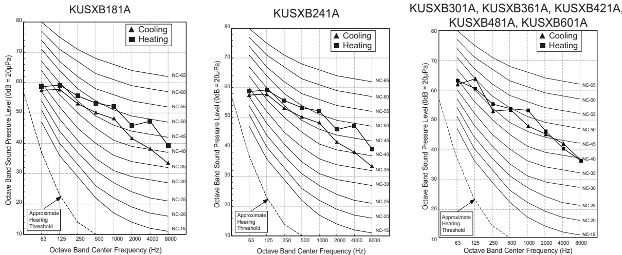
Figure 16: R32 Standard Singe-Zone Systems - A-Coil Outdoor Unit Sound Pressure Level Diagrams.
