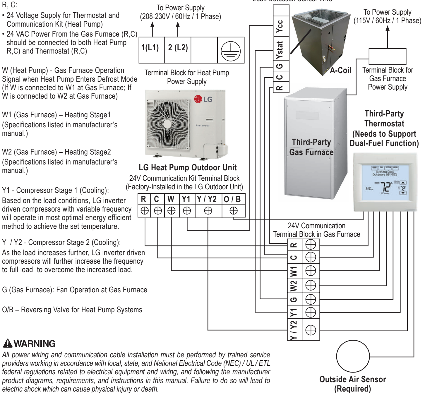
Figure 54: Detailed Two-Stage Wiring Diagram (For Illustrative Purposes Only).
