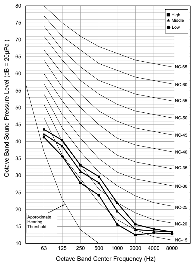
Figure 20: KNSLB121A Indoor Unit Sound Pressure Level Diagram.
