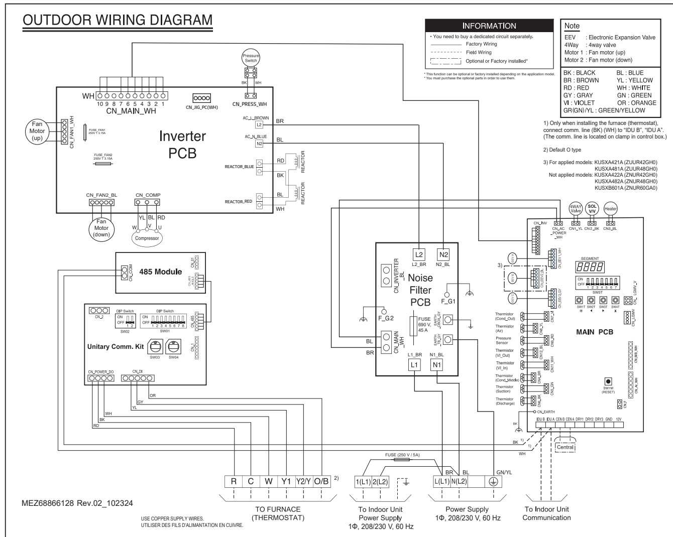
Figure 57: KUSXA422A, KUSXA482A Outdoor Units Wiring Diagram.
