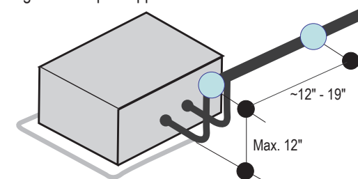
Figure 52: Pipe Support at Indoor Unit.
