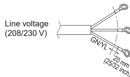
Figure 62: Power Wiring Example.
