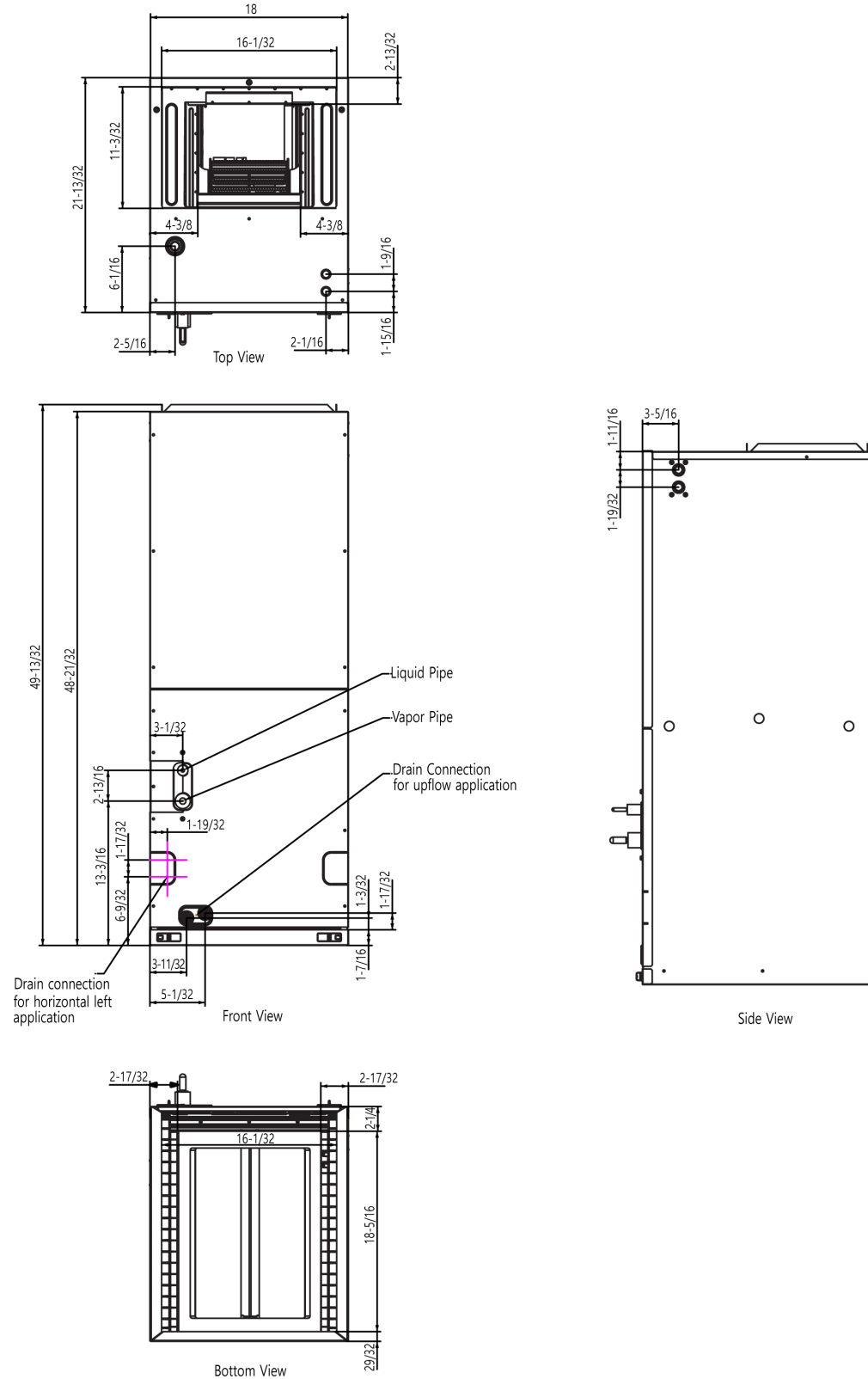
Figure 11: KNSLB121A, KNSLA181A, KNSLA241A Indoor Unit Dimensions.
