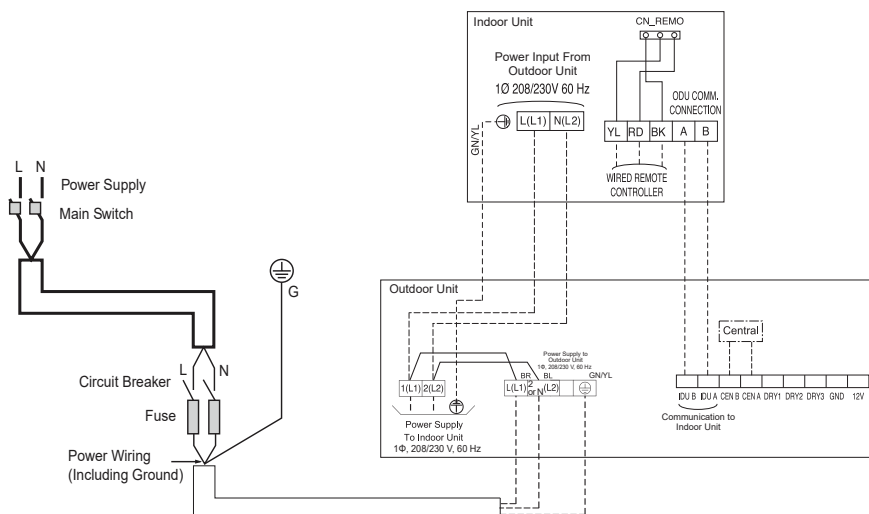
Figure 61: General R32 Single Zone System Power / Communications System Schematic (Appearances May Vary)
