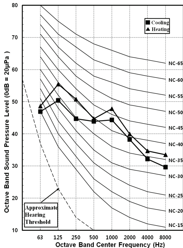
Figure 15: KUSXA121A Outdoor Unit Sound Pressure Level Diagram.
