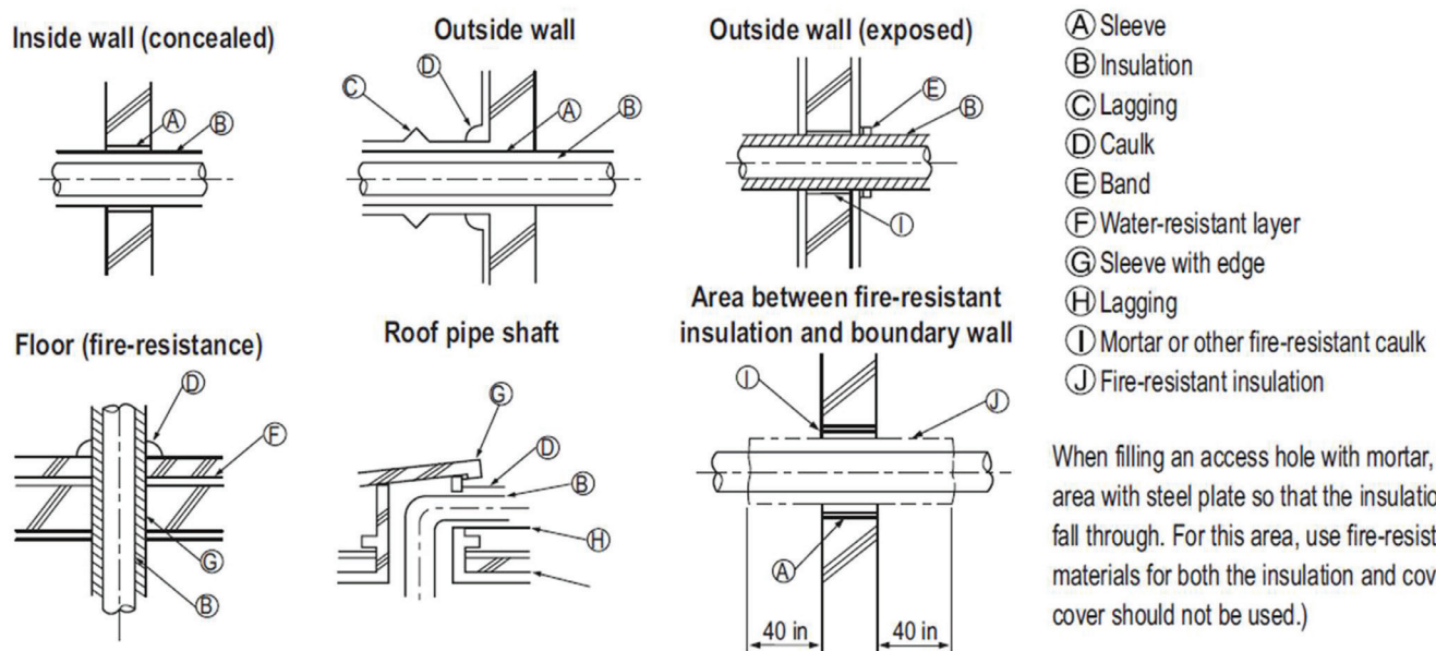
Figure 51: Pipe Sleeve Options.
