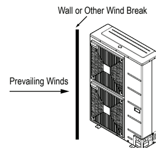
Figure 30: Oceanside Placement Using a Building as Shield, and Placement Using a Windbreak.
