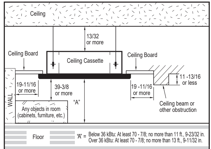
Figure 22: Cassette Indoor Unit Clearance Requirements.
