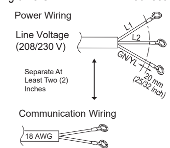
Figure 63: R32 Single-Zone Outdoor Unit to Indoor Unit Wiring and Communications Wiring Diagrams GREATER THAN 130 feet.
