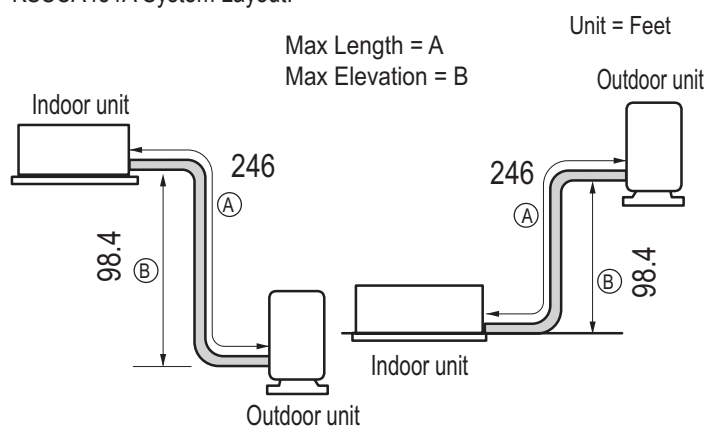
Figure 45: Typical KSSCA301A, KSSCA361A, KSSCA421A, KSSCA481A System Layout.
