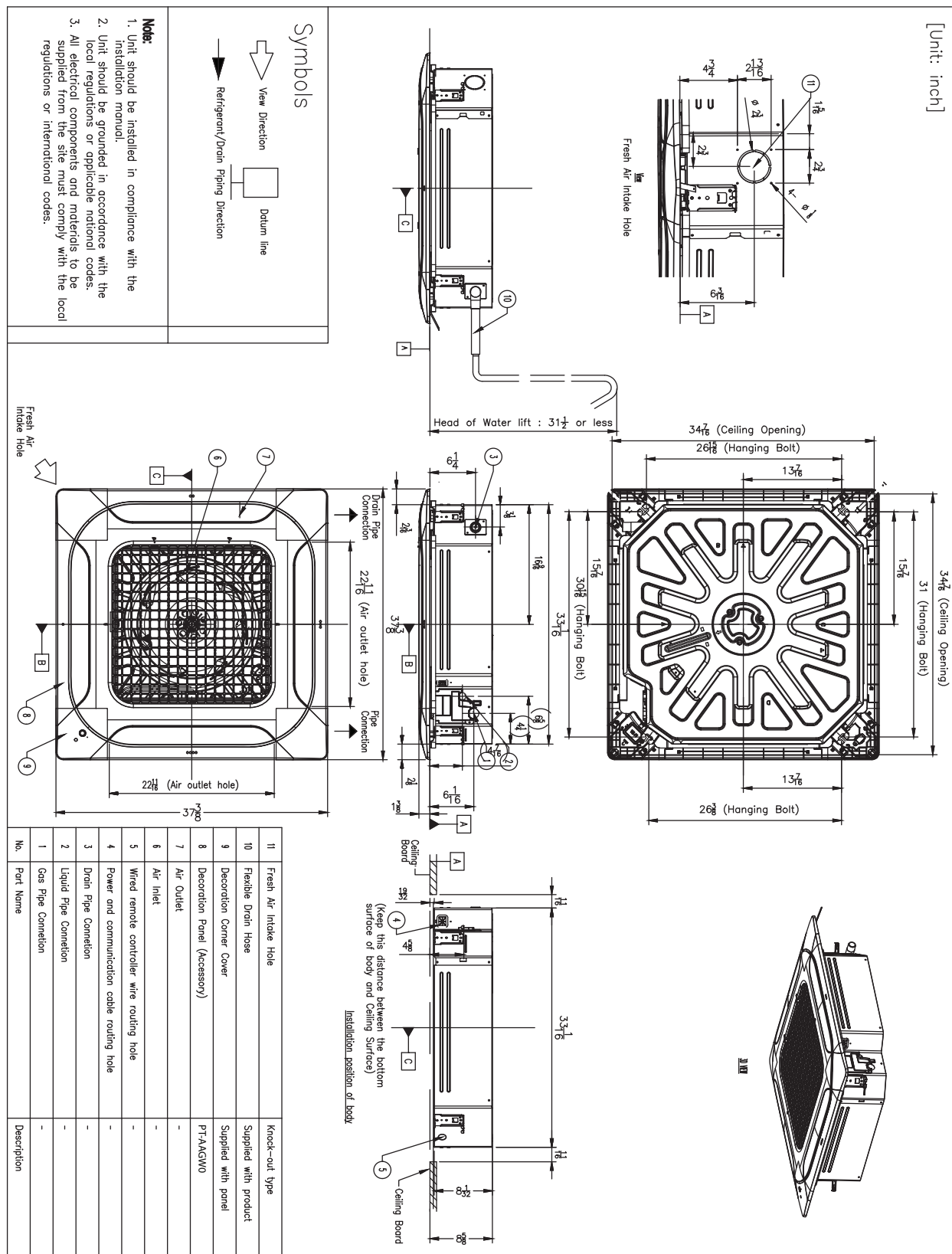
Figure 10: KNSCB241A 3x3 Indoor Unit Dimensions.
