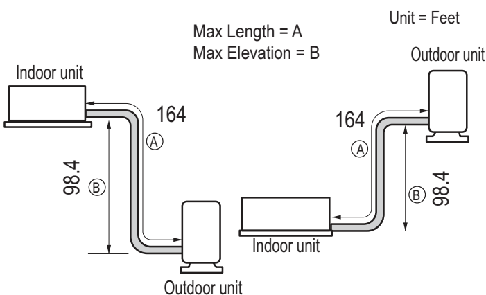
Figure 44: Typical KSUDA181A, KSSCA241A System Layout.
