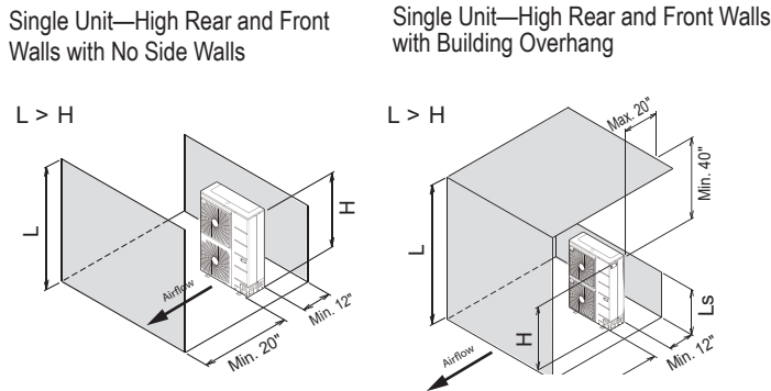
Figure 35: Proper Outdoor Unit Placement and Clearances When There Are Obstacles on the Suction and the Discharge Sides.
