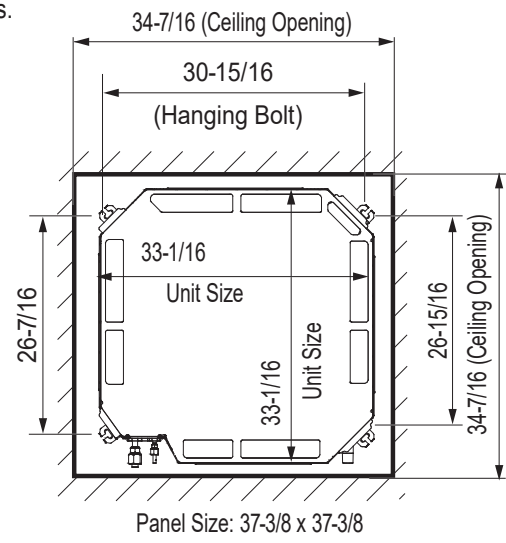
Figure 24: 3 x 3 Cassette Ceiling Opening Dimensions and Bolt Locations.
