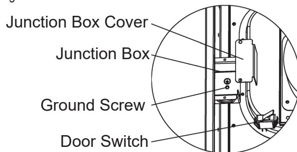
Figure 67: Junction Box.
