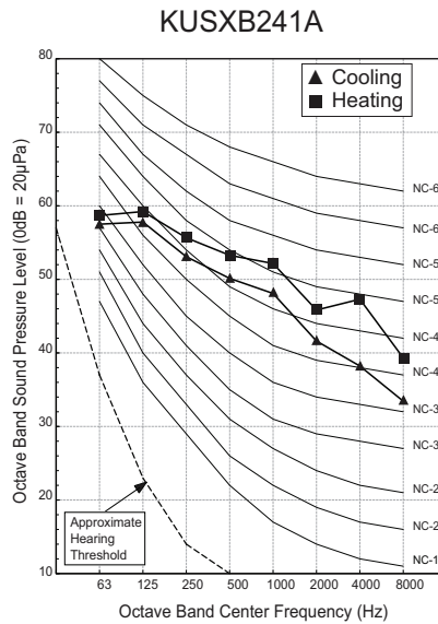
Figure 18: R32 Standard Singe-Zone Systems - A-Coil /Gas Furnace Outdoor Unit Sound Pressure Level Diagrams.
