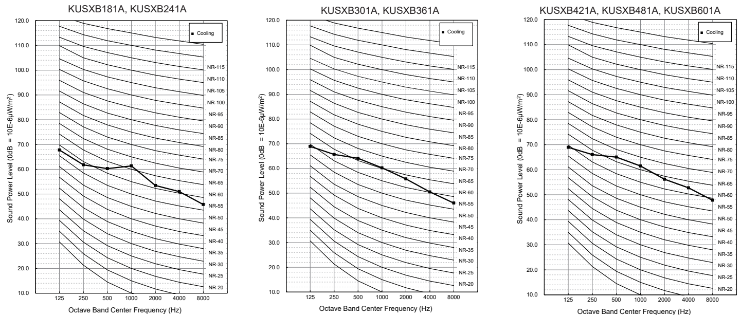
Figure 19: R32 Standard Single-Zone Systems - A-Coil + Gas Furnace Outdoor Unit Sound Power Level Diagrams.
