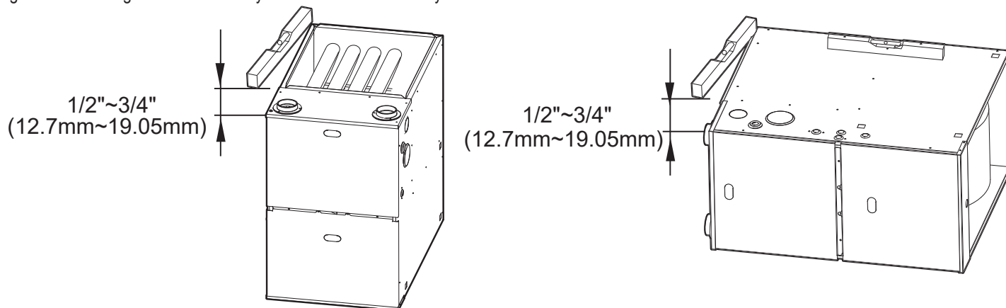
Figure 26: Installing the 96% Efficiency Gas Furnace Horizontally.
