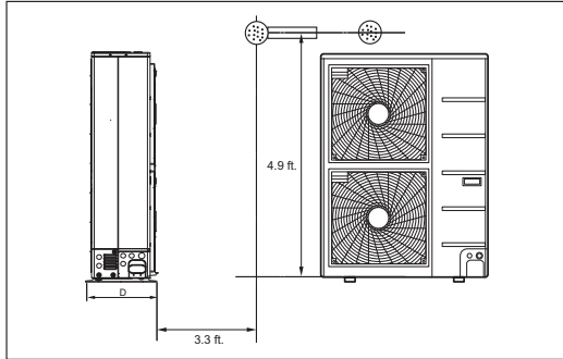
Figure 17: R32 Standard Singe-Zone Systems - A-Coil + Gas Furnace Outdoor Unit Sound Pressure Level Measurement Location (For Illustrative Purposes Only; Appearance Depends on Model).
