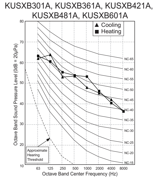
Figure 18: R32 Standard Singe-Zone Systems - A-Coil /Gas Furnace Outdoor Unit Sound Pressure Level Diagrams.
