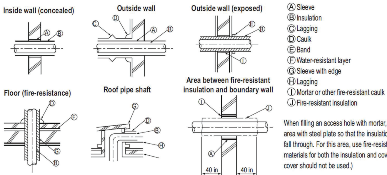
Figure 58: Pipe Sleeve Options.
