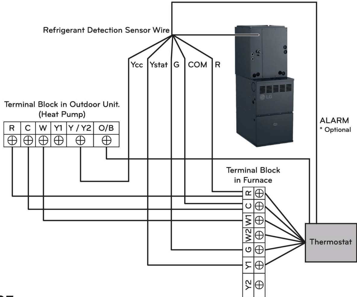
Figure 72: 96% Efficiency Gas Furnace—Wiring Diagram with Dual Fuel One-Stage Cooling, Three-Stage Heating Thermostat.
