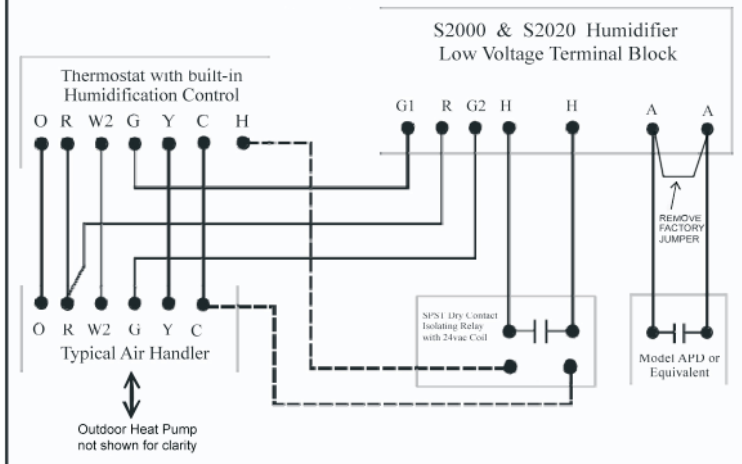
FIG 10 HEAT PUMP SYSTEM AND STEAMHUMIDIFIER WITH COMBO THERMOSTAT/HUMIDIFIER AND ISOLATING RELAY
