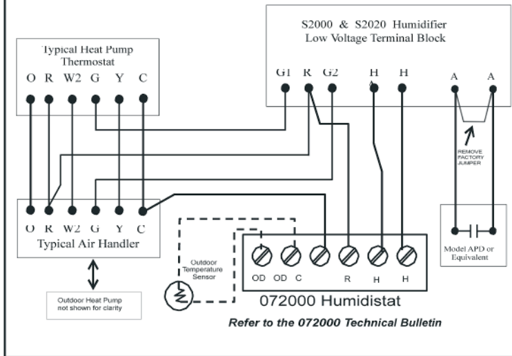
FIG 9 HEAT PUMP SYSTEM AND STEAM HUMIDIFIER WITH 072000 HUMIDISTAT
