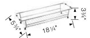
401952 / SOP1721 Laundry rack, Stainless Steel
