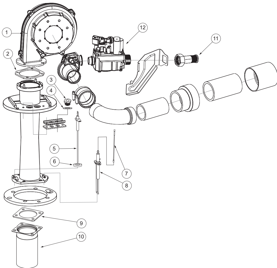
Figure 7. Blower/Burner Assembly
