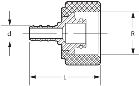
Viega PEX Crimp Port Adapter Zero Lead Brass For ManaBloc Crimp x Port - Model V5039ZL
