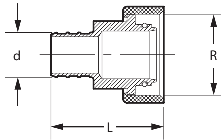
Viega PEX Crimp Supply Adapter Zero Lead Brass For ManaBloc Crimp x Supply - Model V5034ZL
