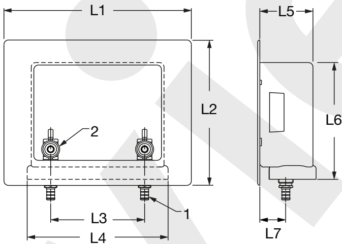
Viega PEX Crimp Outlet Box Zero Lead Brass For Washing Machine 1/4 Turn - Model 2872.9ZL
