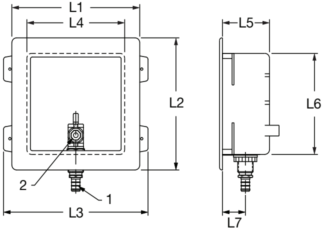
Viega PEX Crimp Outlet Box Zero Lead Brass For Ice Maker 1/4 Turn - Model 2872ZL
