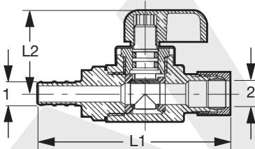
Viega PEX Crimp Stop Valve Straight Zero Lead Chrome Plated Brass Crimp x CTS 1/4 Turn - Model V5026ZL
