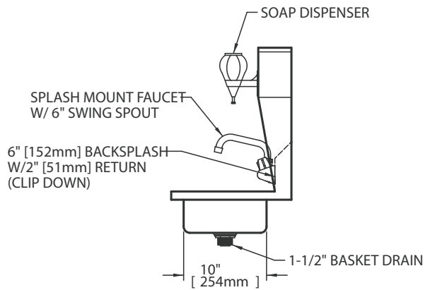
BACKSPLASH DETAIL
