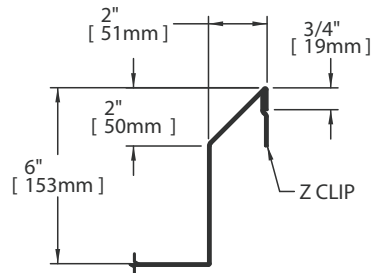
BACKSPLASH DETAIL
