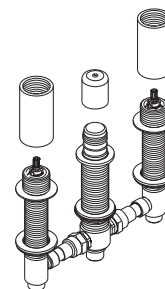
Deck-Mount Bath Faucet Valve
