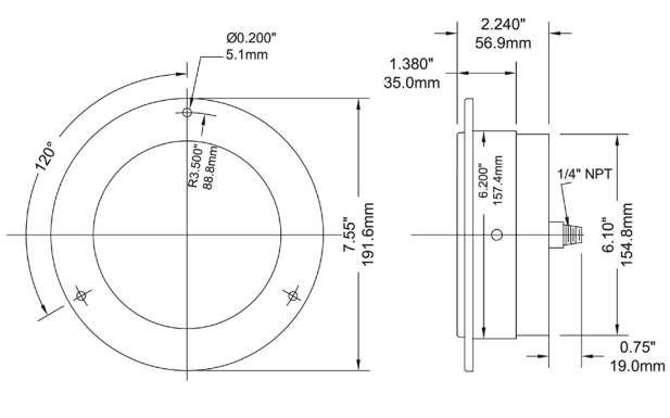
6" Back Connection Stainless Steel with Front Flange
