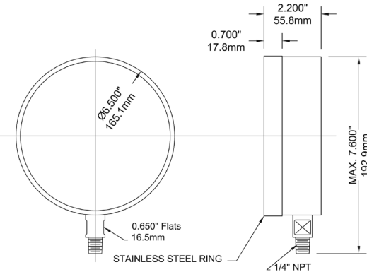
6" Bottom Connection Stainless Steel
