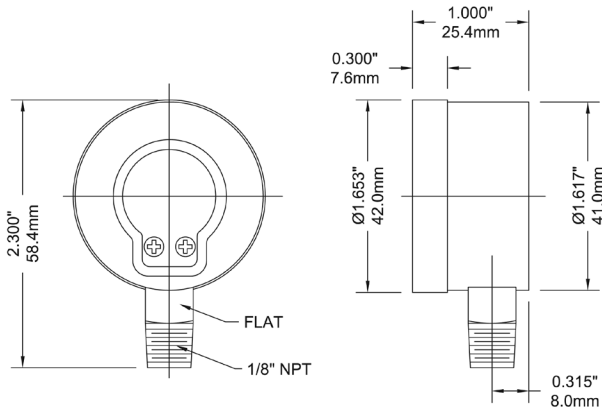
2" Bottom Connection
