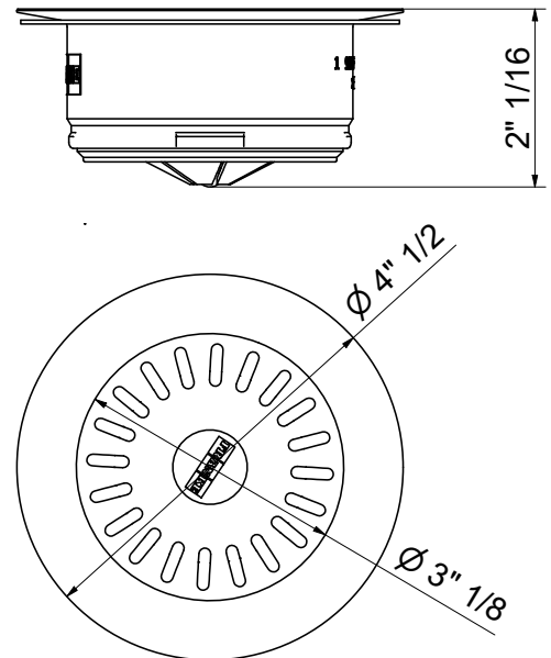
Dimensional Drawing
