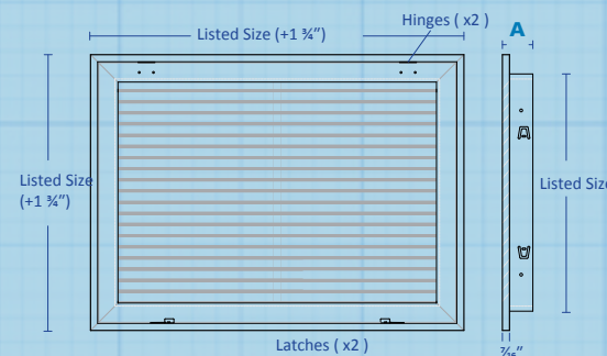
Model 290 14" x 20"
