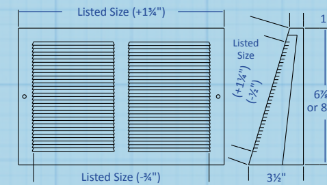
Model 125TR
