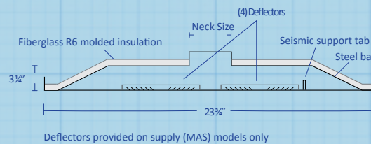
Deflectors provided on supply (MAS) models only
