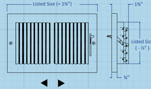
Model 124M
