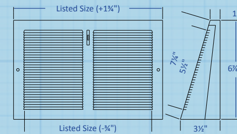
Model 125TS
