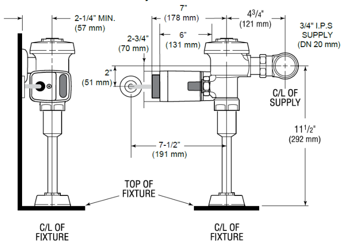
EL-700-A Single-Flush Side Mount Hardwired unit shown on a Royal 186 urinal flushometer
