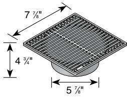
1/4" Grate Opening
