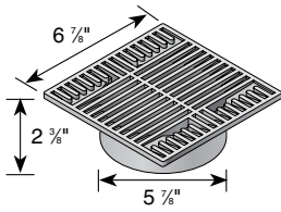
1/4" Grate Opening
