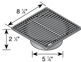
5/16" Grate Opening
