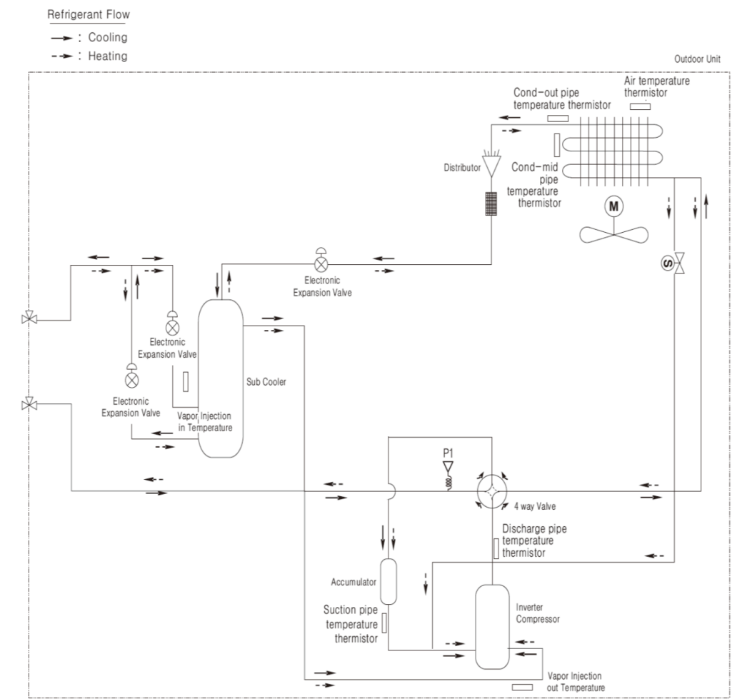
Figure 30: Outdoor Unit Refrigerant Flow Diagrams.
