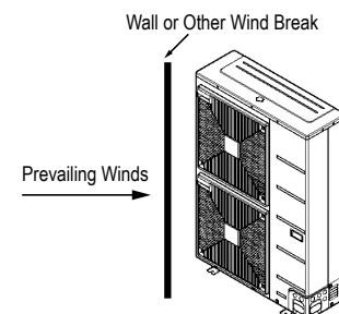
Figure 55: Wind Break.
