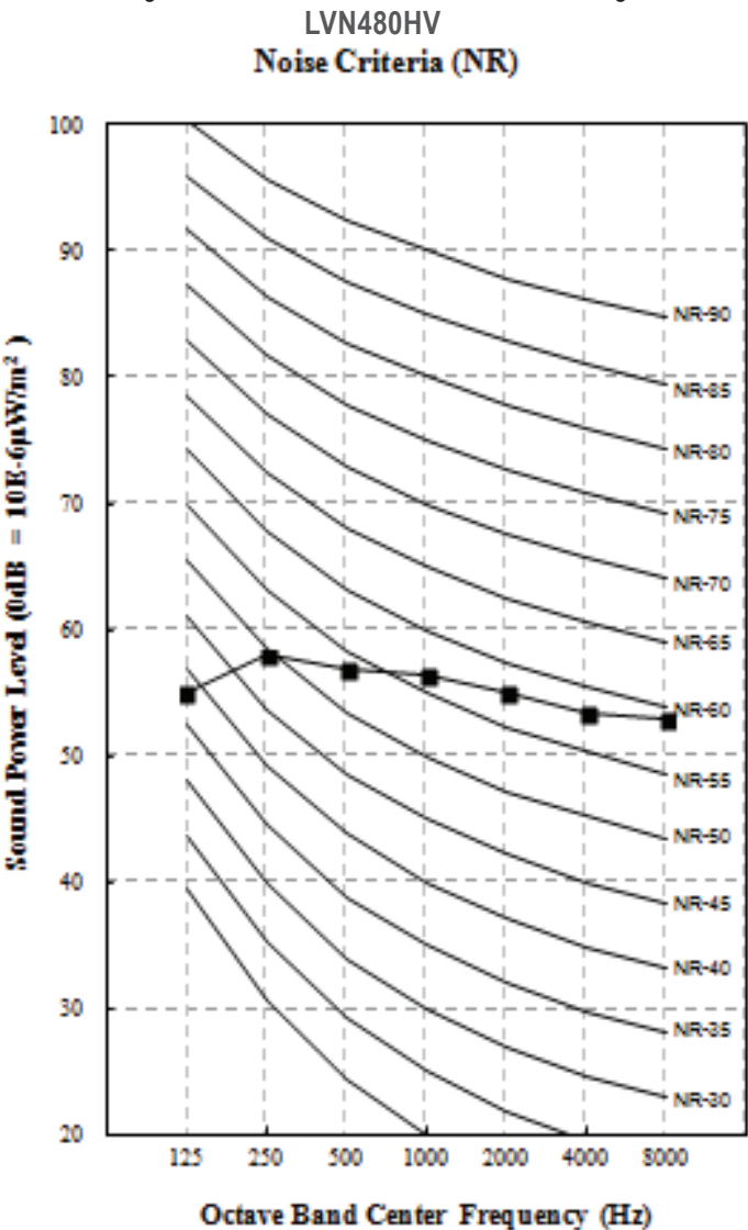
Figure 20: LVN480HV Sound Power Level Diagram.
