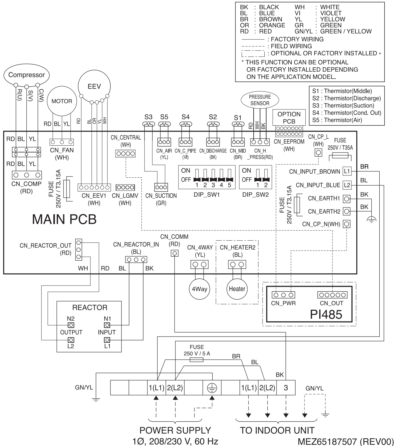
Figure 33: Outdoor Unit Wiring Diagram.
