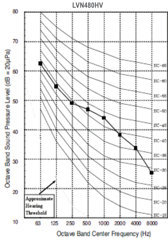
Figure 15: LVN480HV Sound Pressure Level Diagram.
