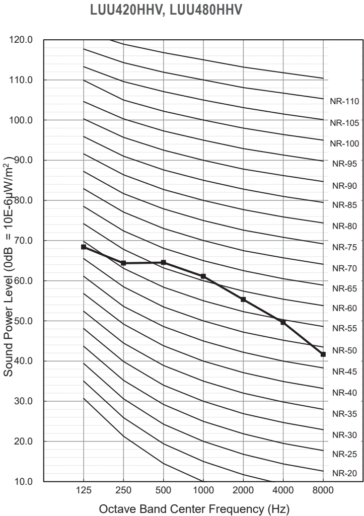
Figure 27: LUU420HHV, LUU480HHV Sound Power Level Diagram.
