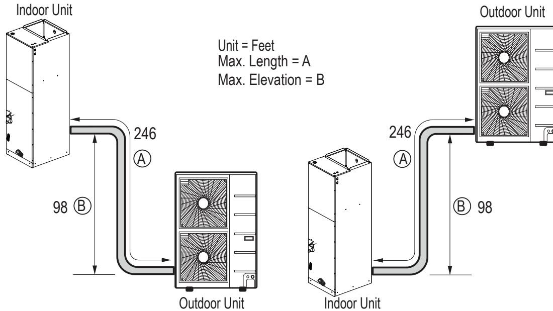
Figure 68: Typical LV361HHV4, LV420HHV and LV480HHV System Layout.
