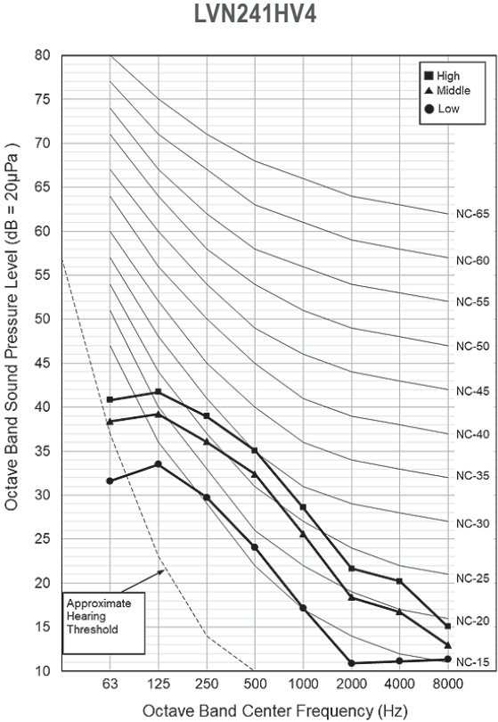
Figure 12: LVN241HV4 Sound Pressure Level Diagram.
