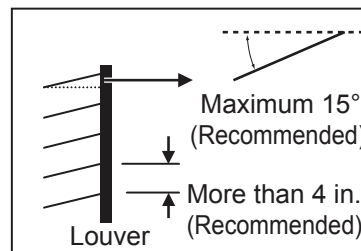
Figure 63: Louver Recommendations.
