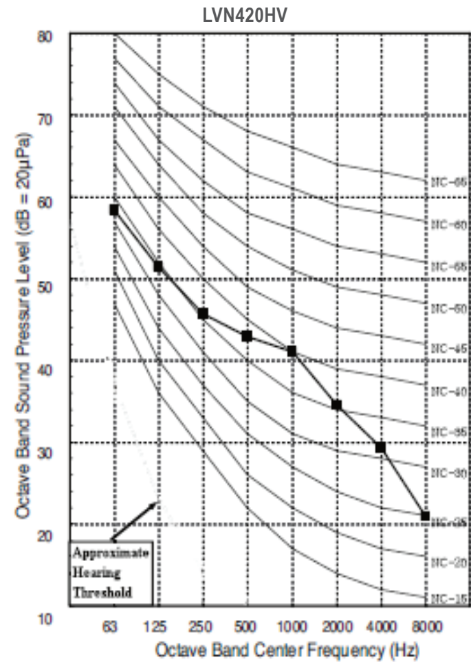
Figure 14: LVN420HV Sound Pressure Level Diagram.
