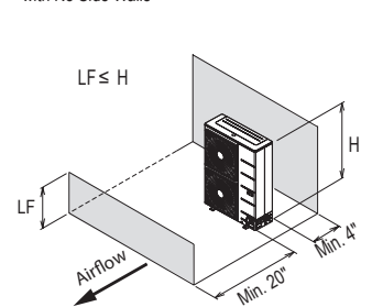
Figure 59: Proper Outdoor Unit Placement and Clearances.
