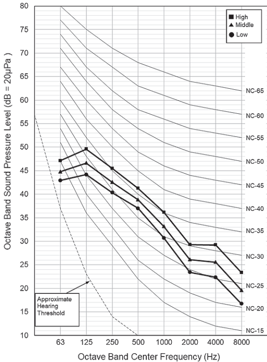
Figure 13: LVN361HV4 Sound Pressure Level Diagram.
