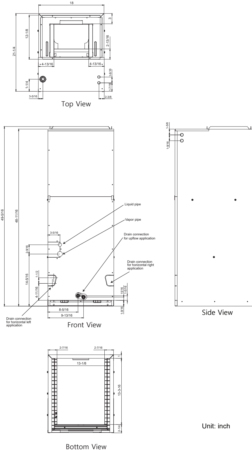
Figure 8: LVN181HV4, LVN241HV4, LVN361HV4 Indoor Unit Dimensions.
