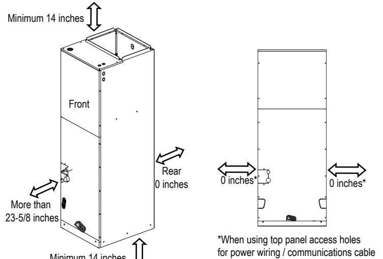
Figure 50: Recommended Clearances for Single Zone LGRED VAHU IDU.
