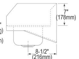
SECTION THROUGH RIM
