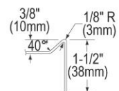
SECTION THROUGH RIM
