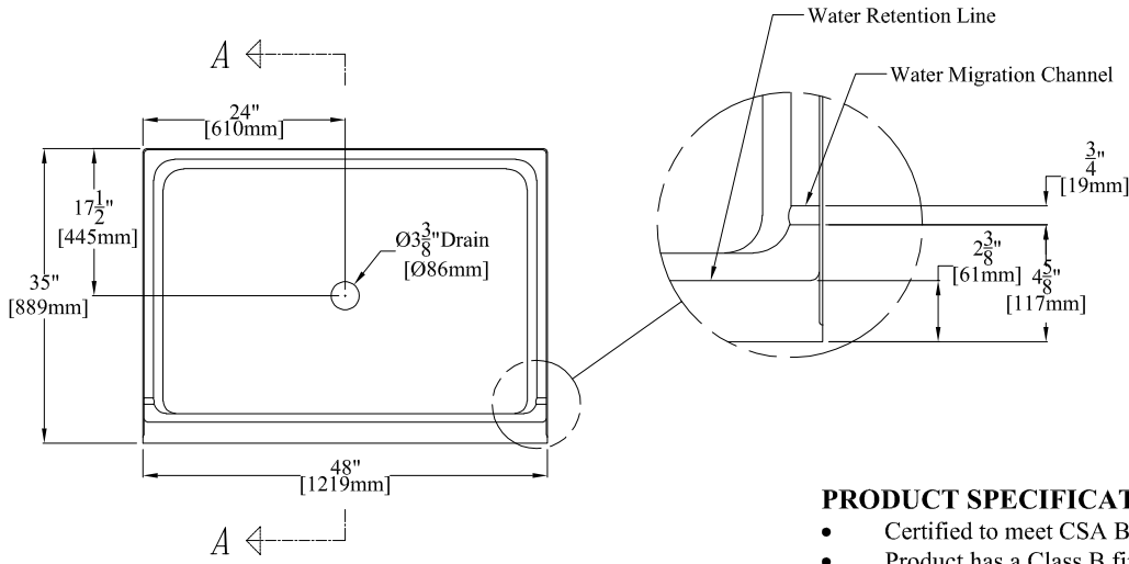
48" x 35" [1219mm x 889mm] Shower Pan w/ 6" [152mm] Threshold
