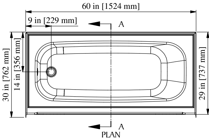
60" [1524mm] Bathtub w/ 19-1/2" [495mm] Threshold
