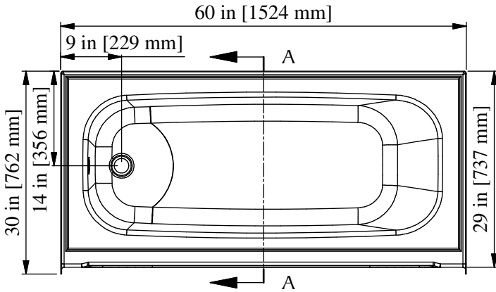
60" [1524mm] Bathtub w/ 18" [457mm] Threshold
