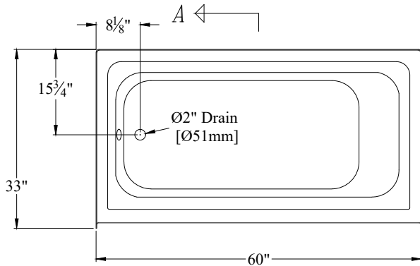
PLAN 60" [1524mm] Bathtub
