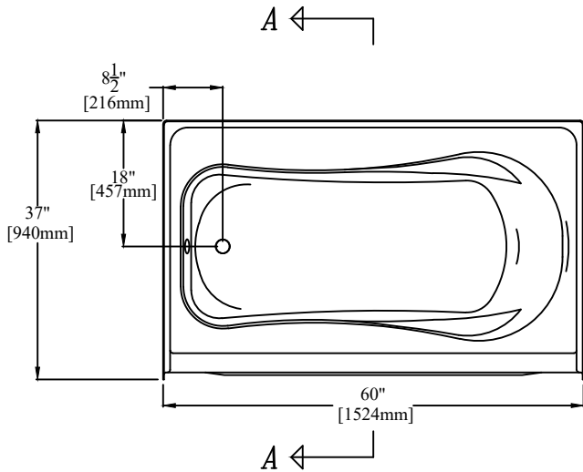
PLAN 60" [1524mm] Bathtub w/ 18" [457mm] Apron, Molded Arm Rests, & Removable Access Panel
