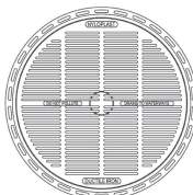
Pedestrian H-20
