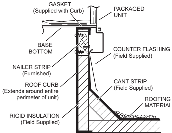
TYPICAL FLASHING DETAIL FOR ROOF CURB
