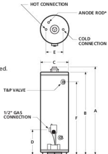
*Location for optional top-mounted T&P Valve if ordered from factory. (FVIR models only)
