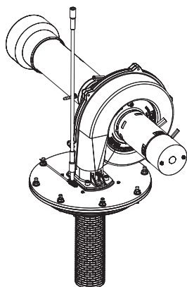
BLOWER/BURNER ASSEMBLY See Page 5
