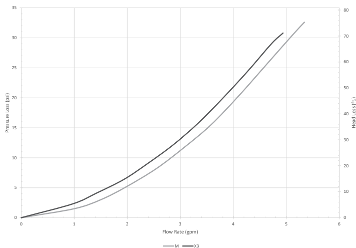
PRESSURE LOSS
