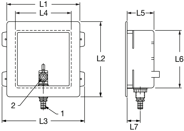
Viega PureFlow Crimp Outlet Box Zero Lead Brass For Ice Maker 1/4 Turn - Model 2872ZL
