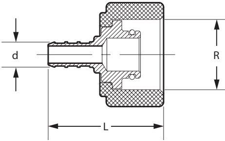
Viega PureFlow Crimp Port Adapter Zero Lead Brass For ManaBloc Crimp x Port - Model V5039ZL
