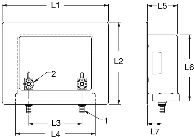
Viega PureFlow Crimp Outlet Box Zero Lead Brass For Washing Machine 1/4 Turn - Model 2872.9ZL
