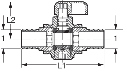
Viega PureFlow Crimp Ball Valve Zero Lead Brass ¼ Turn - Model V5037ZL
