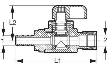
Viega PureFlow Crimp Stop Valve Straight Zero Lead Chrome Plated Brass Crimp x CTS ¼ Turn - Model V5026ZL
