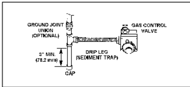
FIGURE 12. GAS PIPING WITH FLEXIBLE CONNECTOR.
