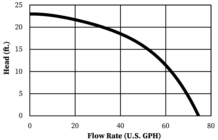
NT1-P Pump Curve
