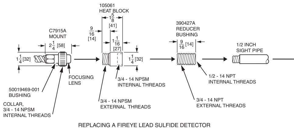
Fig. 1. Mounting dimensions of C7915A Infrared Flame Detector and accessories, in inches. (mm).
