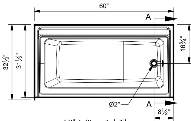
60" I-Piece Tub/Shower w/ 18" Apron & Left or Right Hand Drain
