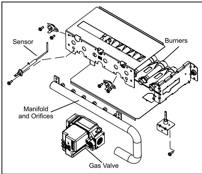
Figure 4. Manifold Gas Valve Assembly (A93, A95, 92G1, 95G1 & 96G1)
