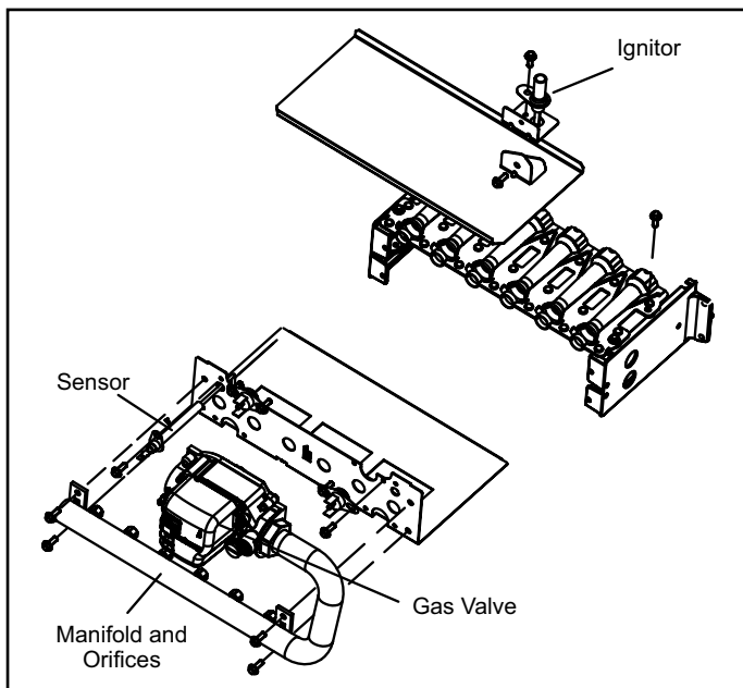
Figure 5. Manifold Gas Valve Assembly (A80 & 80G1)
