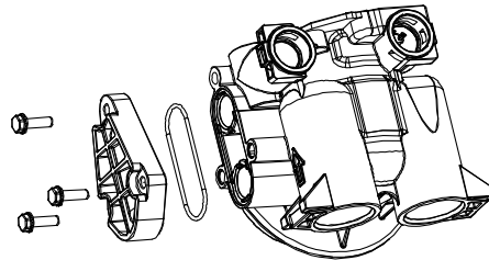
85UF Valve
