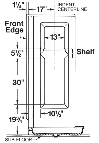
Valve Placement Dimensions
