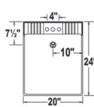
Top Views
