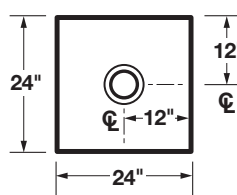
Top Views
