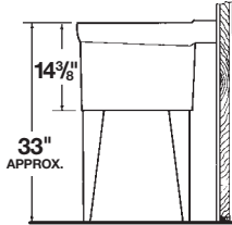
Side Views
